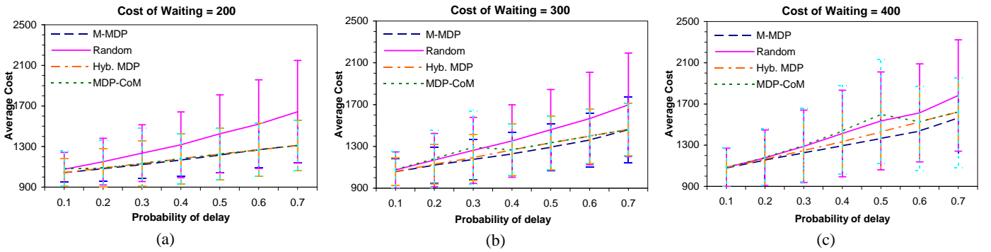
Figure 10: Line plots showing the average costs incurred for increasing probabilities of the order being delayed and increasing costs of waiting for the order in response to the delay.
