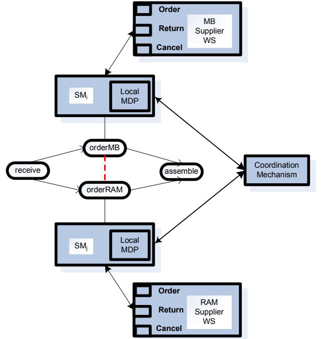
Figure 7: Each service manager locally decides its action in response to the exogenous events. The service managers coordinate using a coordination mechanism that each observes perfectly.
