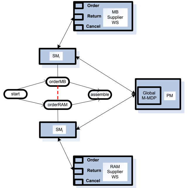
Figure 3: The process manager does the global decision making for adaptation using the M-MDP model. We do not show the constraint analysis module here for clarity.
